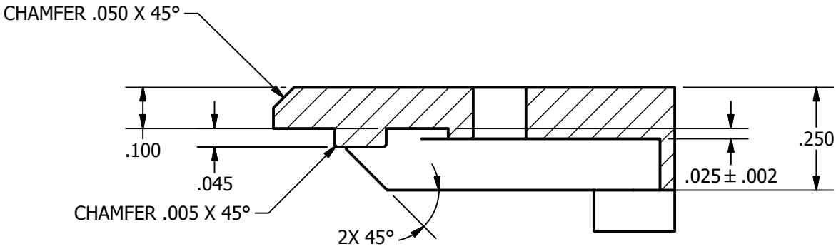
SECTION B-B
